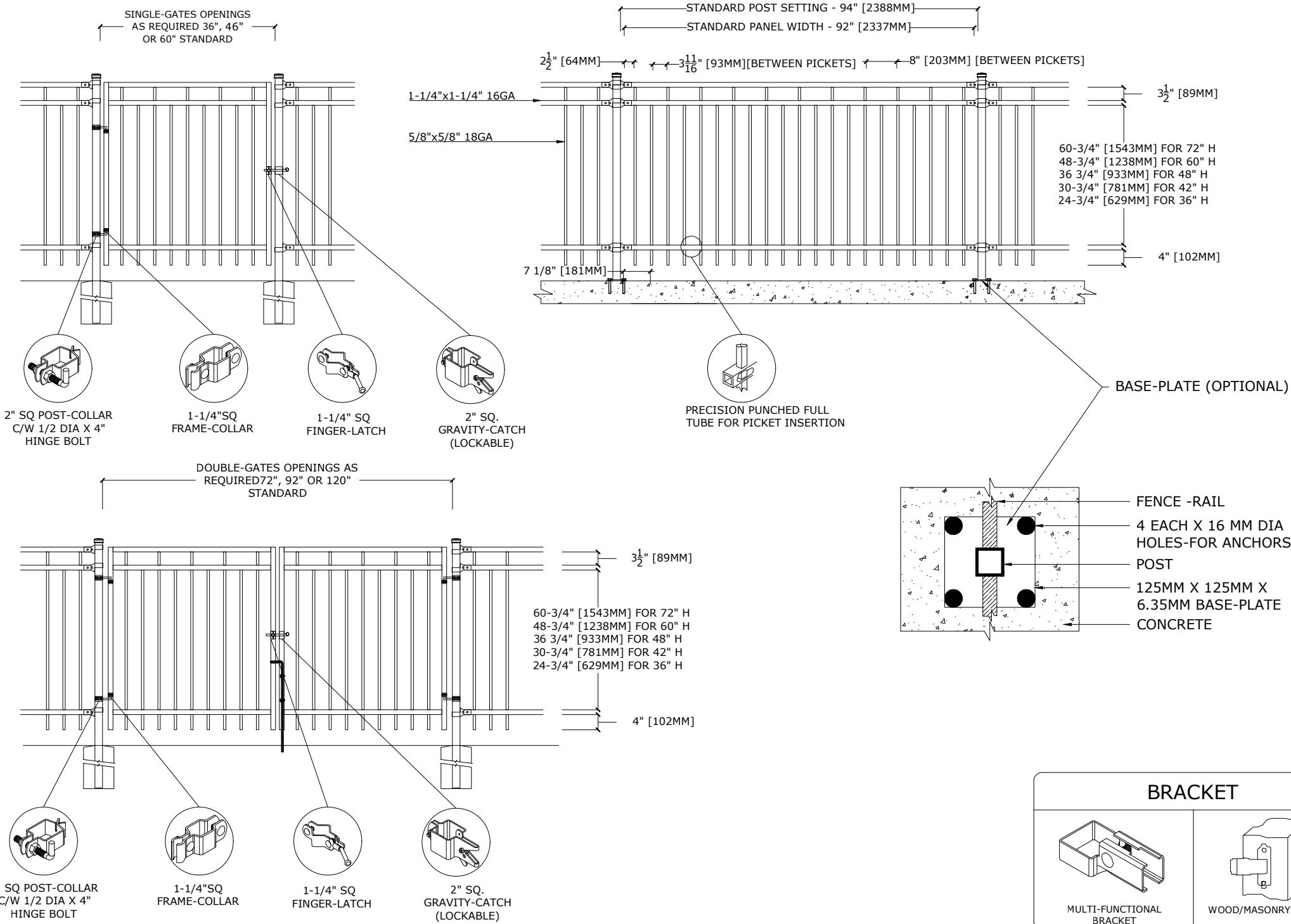
MULTI-FUNCTIONAL BRACKET
